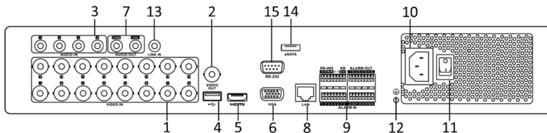
Figure 1. 12 DS-7316HQHI-SH and DS-7316HGHI-SH
