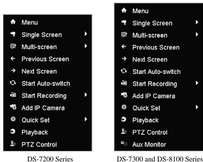
Figure 3.1 Right-click Menu
