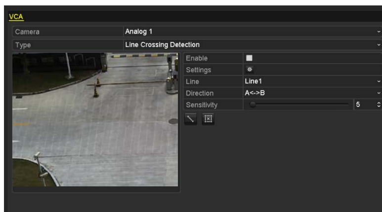
Figure 5. 19 VCA Settings
